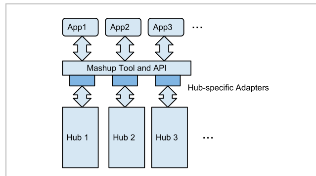
Figure 2. Mashup Platforms used to address WoT hub interoperability.
