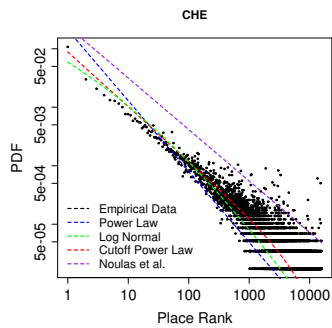
Figure 1: PDF of rank-distance on log-log scale for Switzerland. (Best viewed in color)
