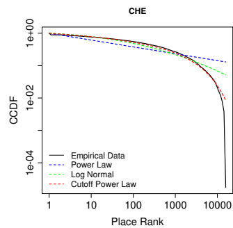
Figure 3: CCDF of rank-distance on log-log scale for Switzerland. (Best viewed in color)
