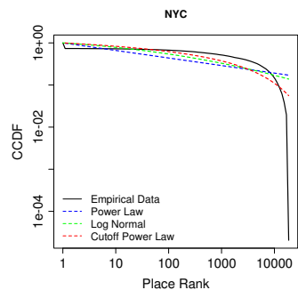
Figure 4: CCDF of rank-distance on log-log scale for NYC. (Best viewed in color)
