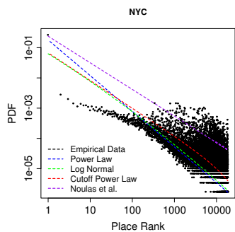
Figure 2: PDF of rank-distance on log-log scale for NYC. (Best viewed in color)
